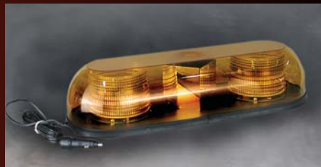
05C-720 Amber Emergency Light Bar 23" wide, 6 1/2" high, 4 x 75 lb. pull magnet, 15' straight cord with cigarette lighter plug, built in on/off switch. 12 x 24V.
