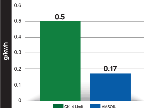
Oil Consumption
