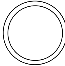
CR-50-52H Wound Kraft EB-52, engine block for 29mm motors ID 0.978, OD 1.14
