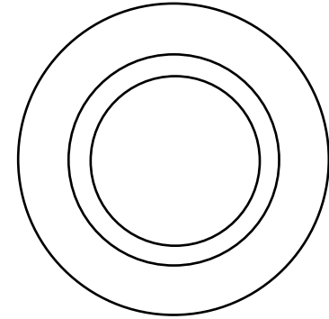
CR-50/52H-1.88P Light Ply ID 0.978/1.215, OD 1.798
