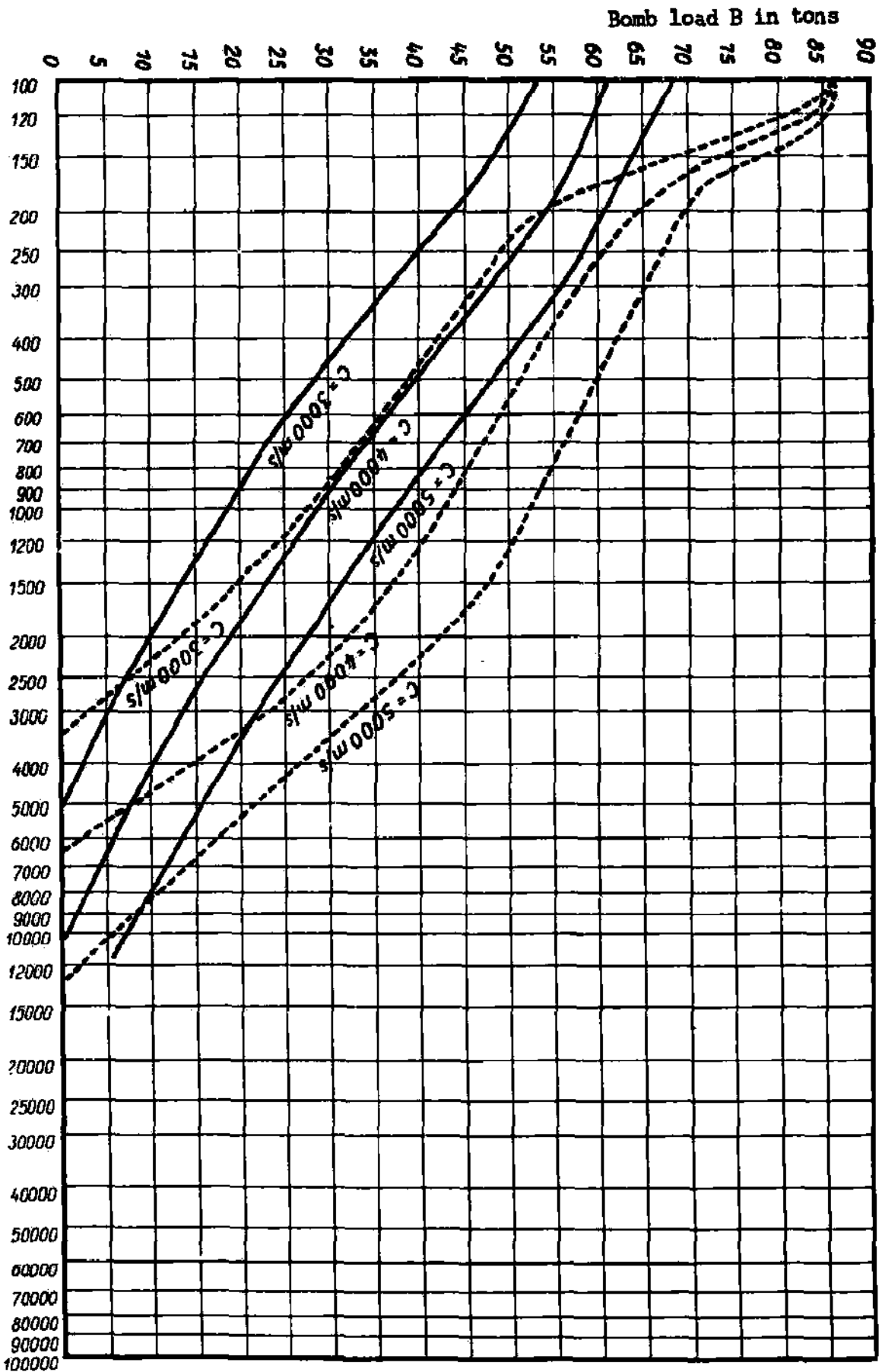
Fig. 82: Comparison of the ranges and of the Rocket Bombers with equal bomb loads for c = 3000 , 4000 and 5000 \text{ m/sec} . If the return to the launching point is effected by a full speed gliding turn (solid lines), or second, if there is a slower gliding turn, followed by a second rocket acceleration (dotted lines).
