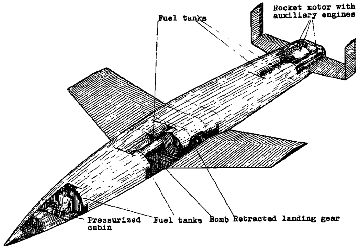
Figure 33; Total view of 10 ton Rocker Bomber
