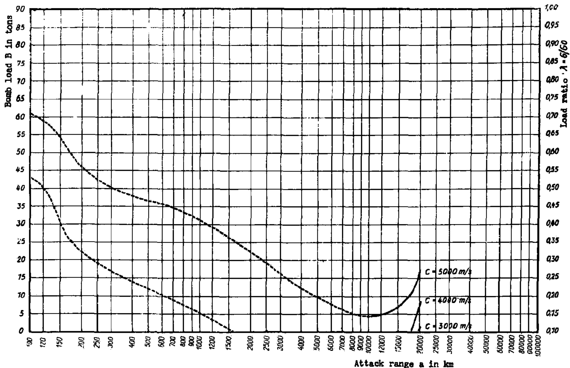
Fig. 96: Relationship between attack range a and bomb load B , i.e. load ratio \lambda , in the case of point attack with double propulsion and landing at the antipodal point for c = 3000, 4000 and 5000 \text{ m/sec} .
