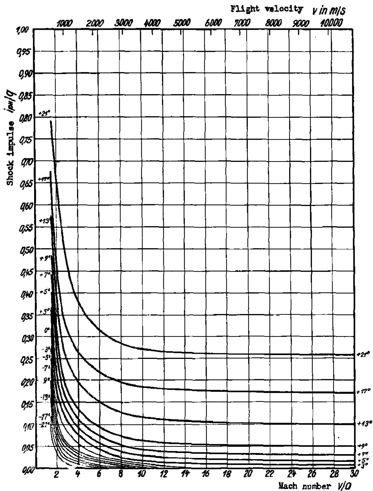
Fig. 43: Coefficients ipw/q of a shock impulse perpendicular to a flat plate for various flight velocities v and angles of attack \alpha in an atmosphere of 86% N_2 and 14% O_2 and density \rho = 10^{-7} \text{ kg sec}^2/\text{m}^4 (molecular flow region).
