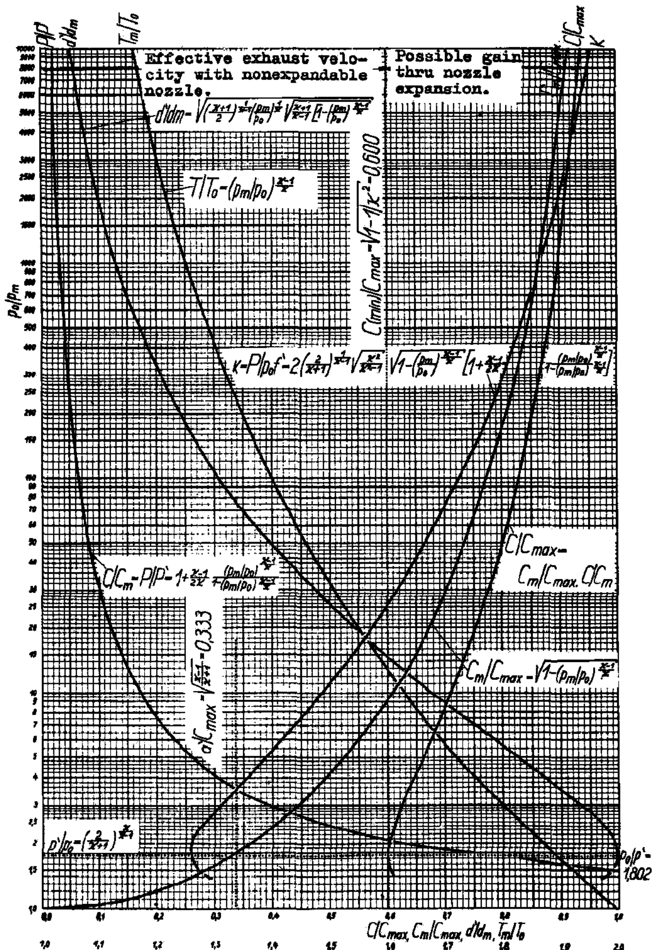
Figure 16; Firegas flow with x=1.25 K = P/p_0 C/C_m = P/P'
