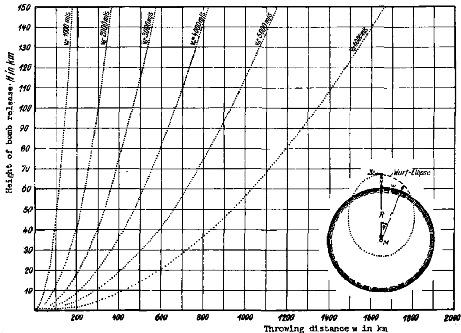
Fig. 87: Throwing distance of surface bomb according to second approximate calculation. (Path as a Kepler ellipse, taking into consideration the Earth's curvature, and also the approximate air resistance) See p. 130.
