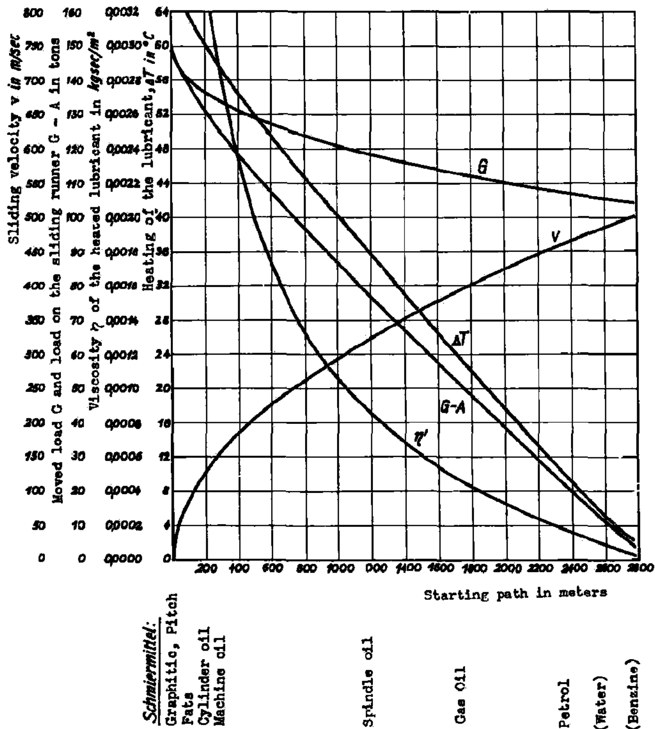
Fig. 55; Sliding velocity v , moved load G , loading on the runners G-A , heating of the lubricating film \Delta T , viscosity \eta of the heated lubricating agent, and practical manner of lubricating for various points along the starting path.
