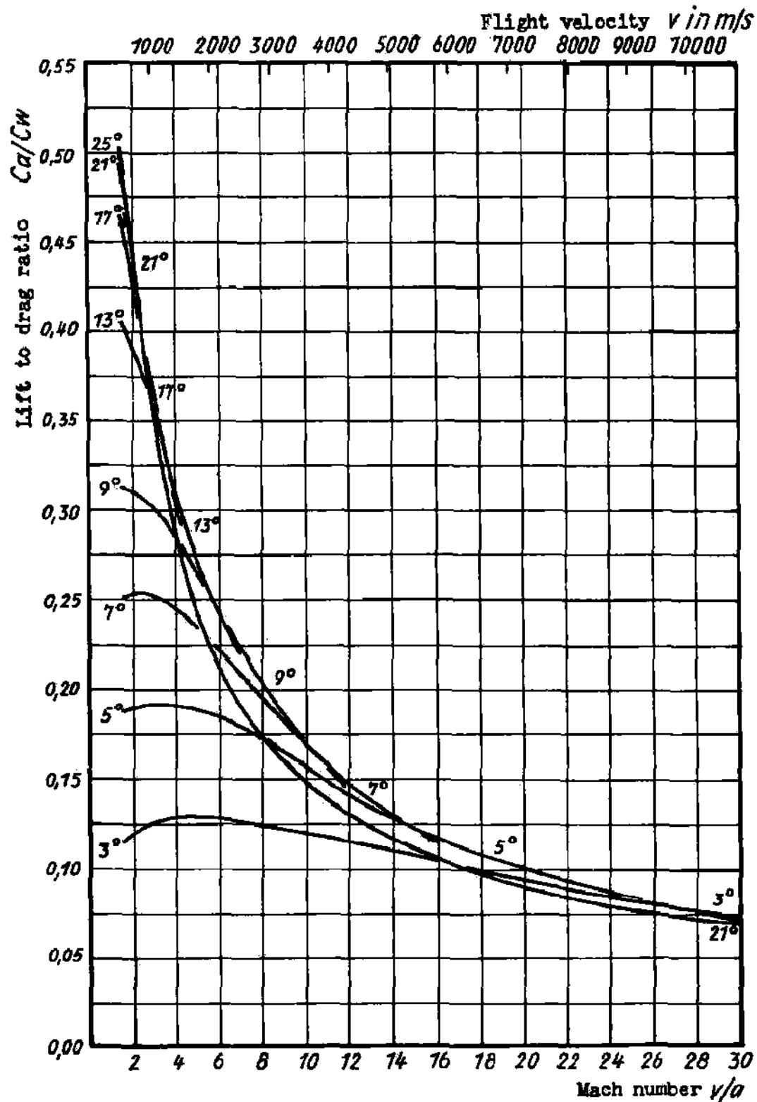
Fig. 46: Lift to drag ratio of a flat infinitely thin plate in molecular flow region.
