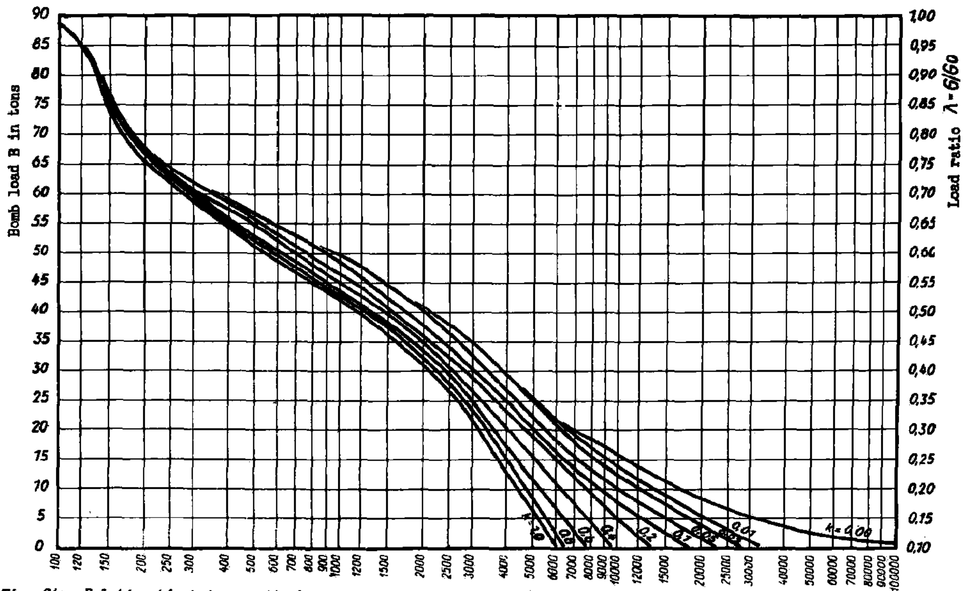
Fig. 94: Relationship between attack range a , and return range k.a and bomb load B , that is load ratio, in case of a point attack and a second propulsion at the knee of a dog leg path to a secondary base, c = 4000 m/sec. (see p. 138, sec. 3)
