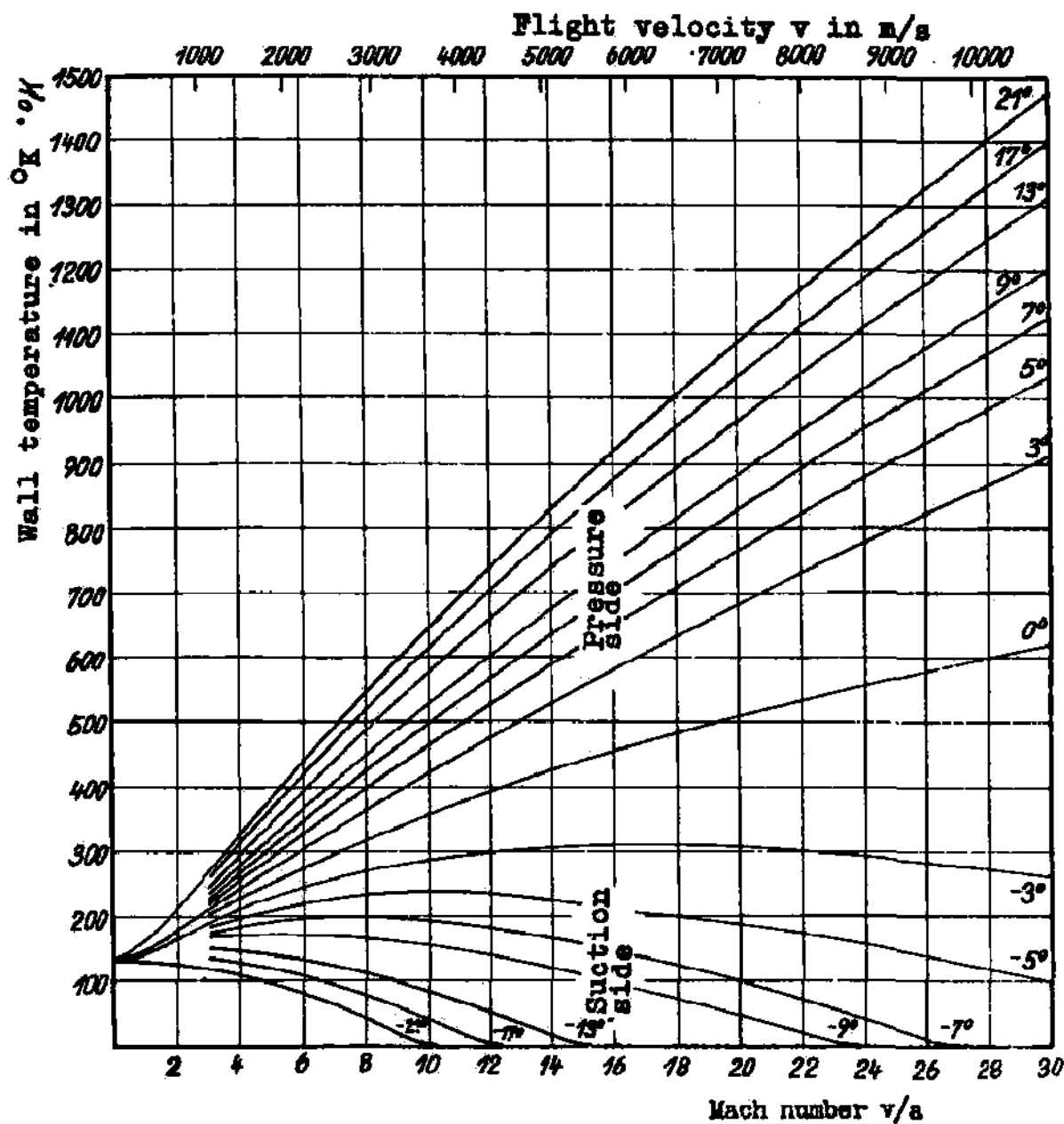
Fig. 42: Surface temperature of a flat plate in an atmosphere of 86% \text{N}_2 and 14% \text{O}_2 and with density \rho = 10^{-7} \text{ kg sec}^2/\text{m}^4 (in molecular flow region) for various flight velocities v/a and various angles of attack \alpha
