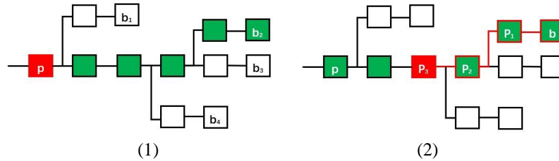
Fig. 4 Process of determining the main branch (1) and save point generation (2)
