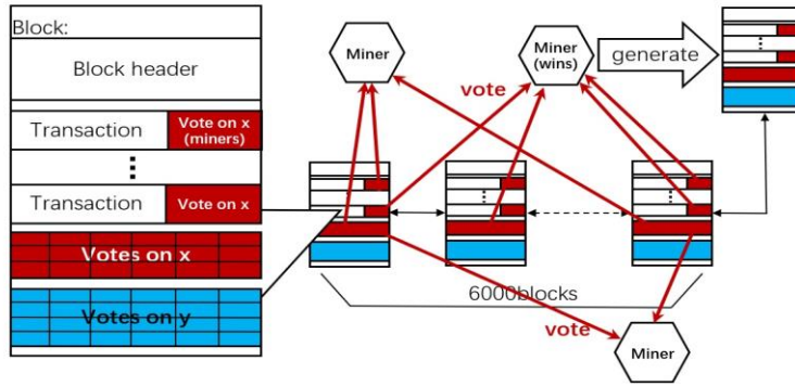
Fig. 2. Process of block competition
