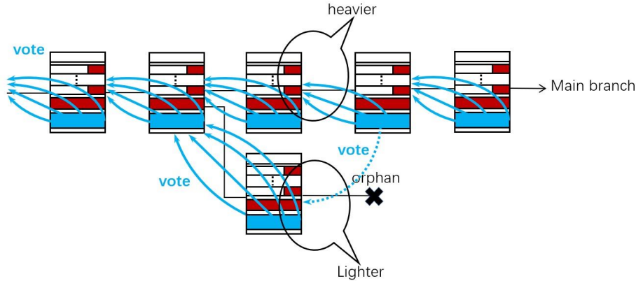
Fig. 3. Process of main branch selection
