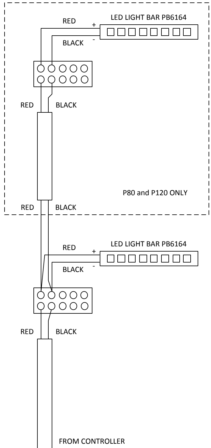
CONNECTIONS ON P2.0 MACHINES MANUFACTURED AFTER OCT 2013
