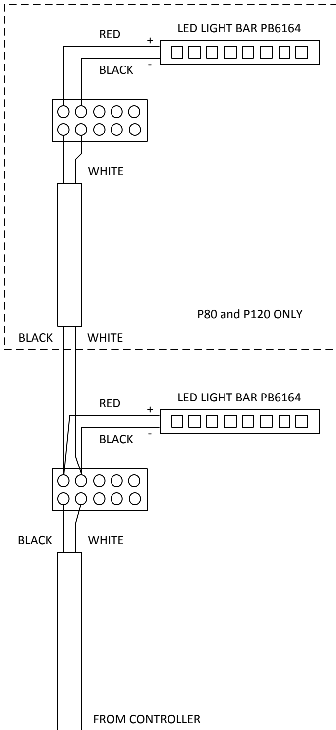
CONNECTIONS ON P2.0 MACHINES MANUFACTURED PRIOR TO OCT 2013
