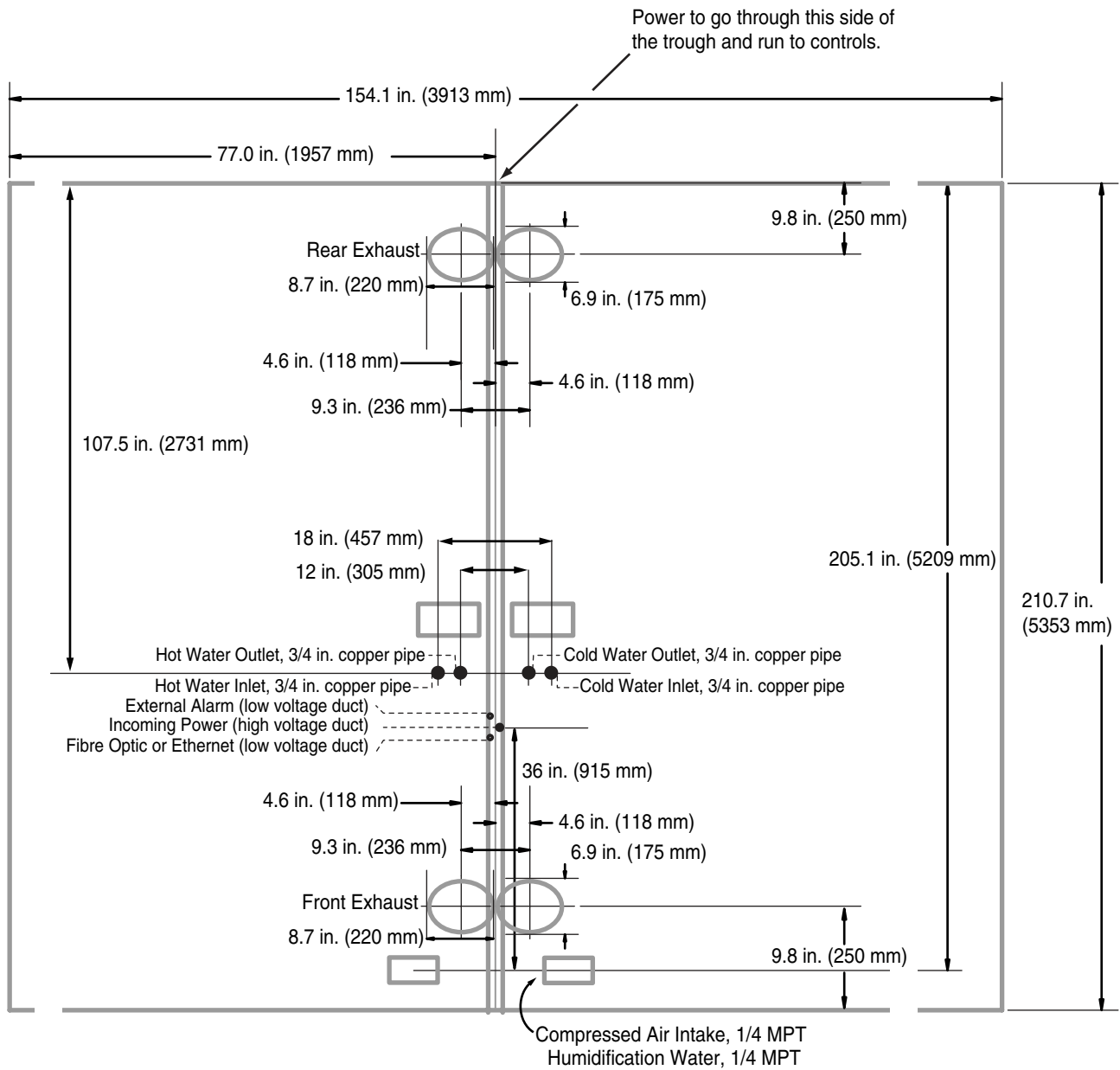
Top view of P80 incubator showing service locations
