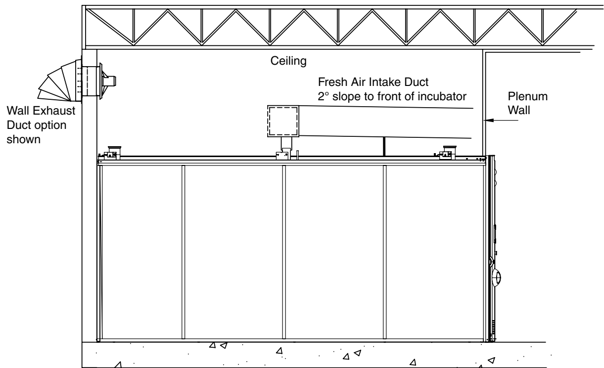
P80 Fresh Air Intake Duct - side view
