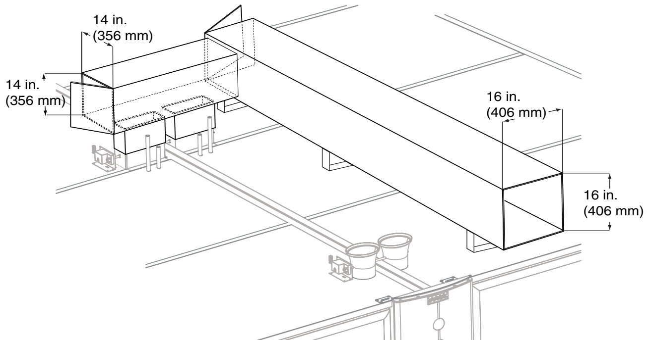
P80 Fresh Air Intake Duct Assembly - Both ducts require clean out hatches. Large duct must slope two degrees (2°) towards the front of the incubator.
