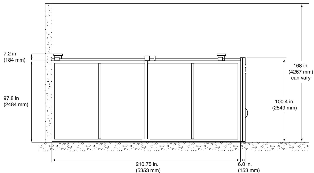
Side view of P80 incubator cabinet
