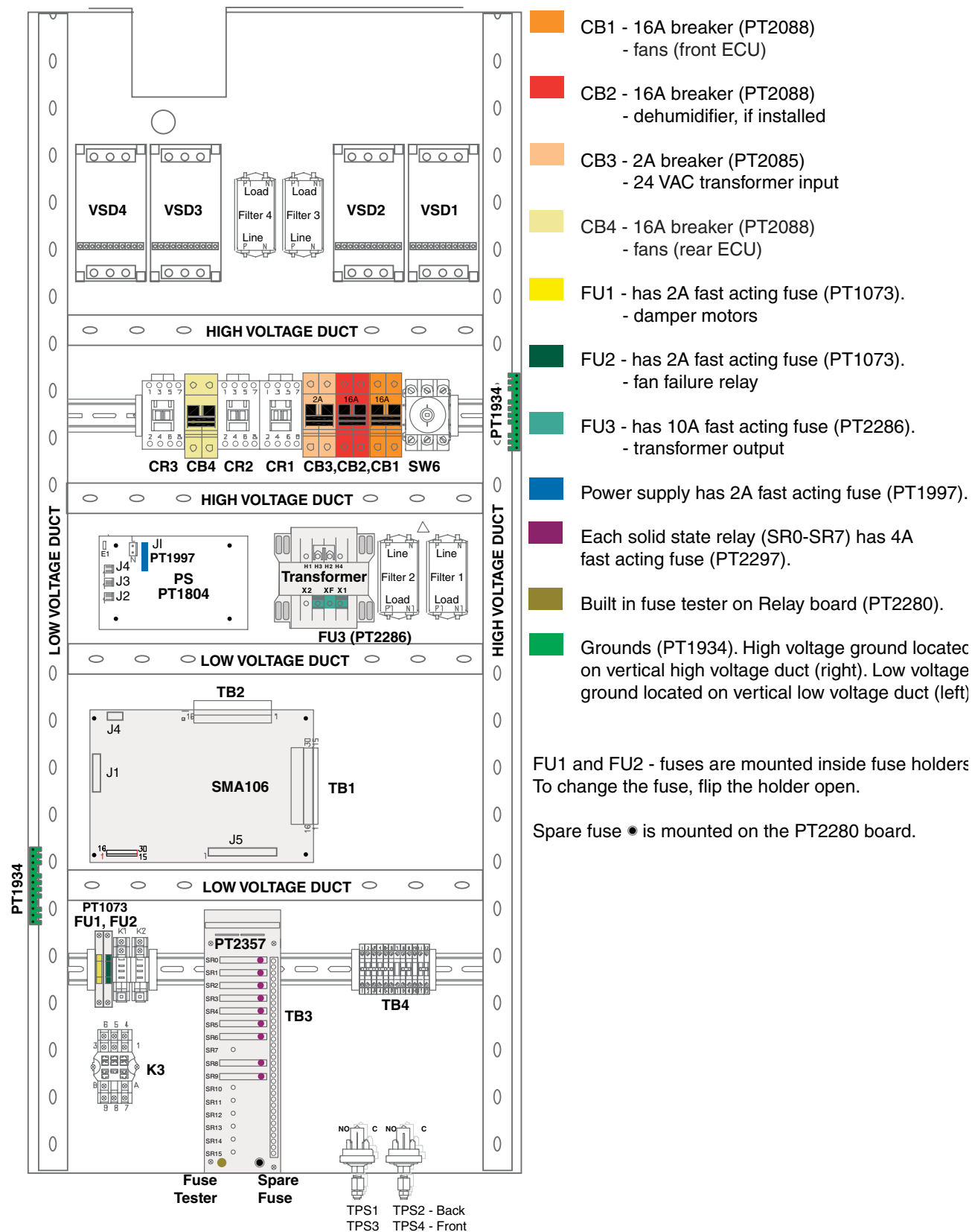
Control Box, P80 Incubators - location of circuit breakers and fuses
