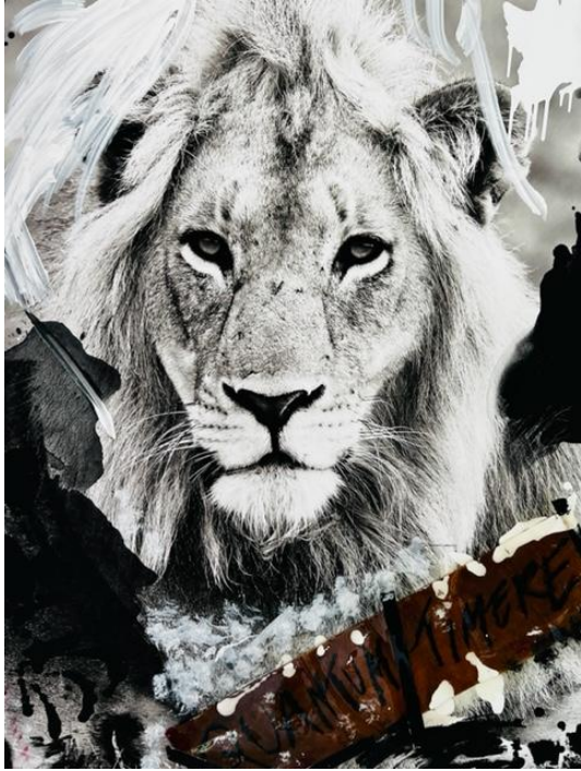
Quantum Timere
